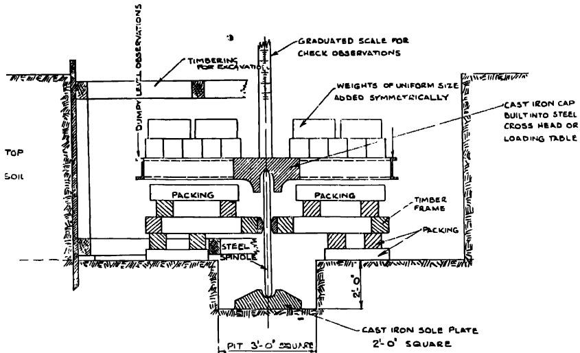
Fig. 19.—Method of Testing Bearing Capacity of Ground.
